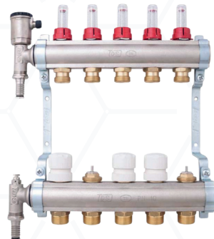
COLLECTOR WITH FLOW AND THERMOSTAT CONTROL
