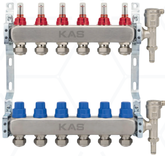
COLLECTOR WITH FLOW AND THERMOSTAT CONTROL
